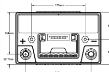
ODX-AGM34M LEFT POSITIVE DUAL TERMINALS (SAE & STUD)
